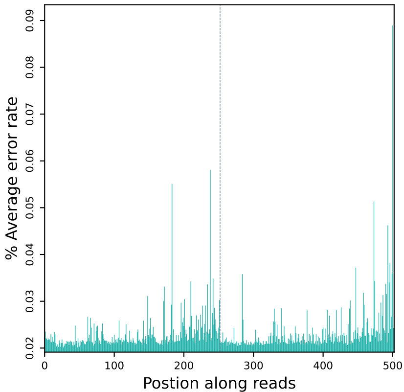
Error rate distribution along reads (R10826)
